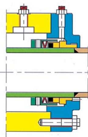
Single end mechanical seal 单端面机械密封
