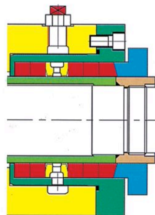
Packing seal 填料密封
