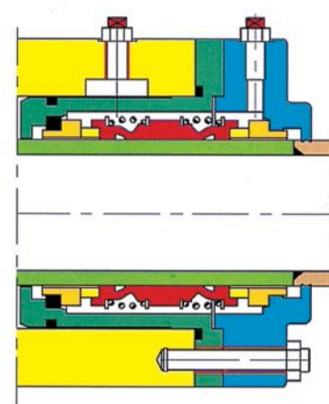
Double-end mechanical seal 双端面机械密封
